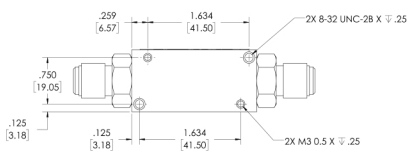
C-SERIES MFM RS485/ANALOG VERSION WITH 4VCR FITTINGS
