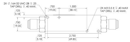
1/4" TUBE MODBUS MFM STD SIZE VERSION
